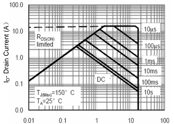
Figure 4 Safe Operation Area
